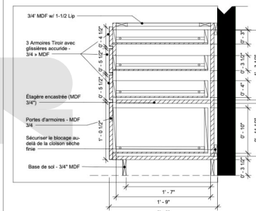
4 Details - Cuisine M3 1 1/2" = 1'-0"
