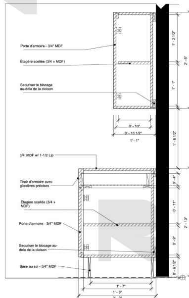
3 Details - Cuisine M2/M4.M5 1 1/2" = 1'-0"
