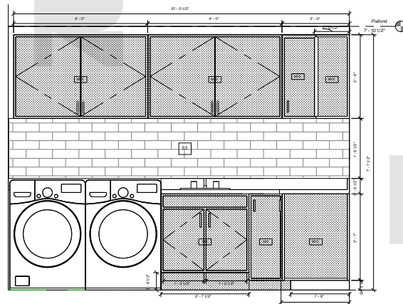
1 Elévation S.Lavage - 1 1" = 1'-0"
