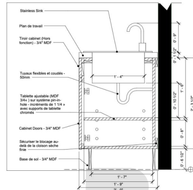
2 Details - Cuisine M2 Evier 1 1/2" = 1'-0"
