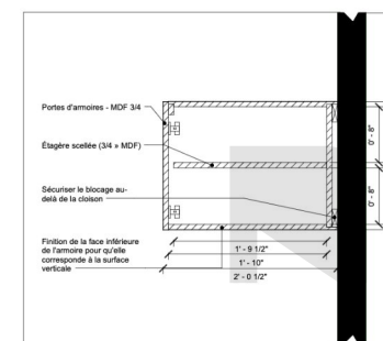
4 Details - Cuisine M3 1 1/2" = 1'-0"
