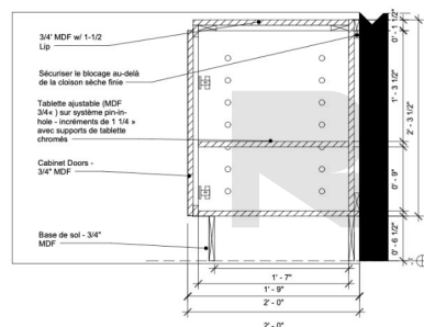
1 Details - Cuisine M1 1 1/2" = 1'-0"
